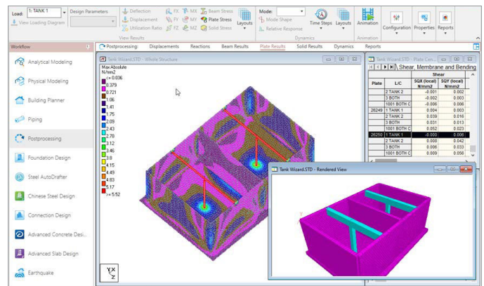
Design water tank structures using STAAD.Pro and STAAD Advanced Concrete Design.
